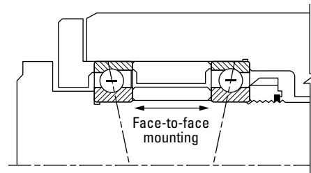
Fig. 127. DF Mounting, fixed (not suggested).
